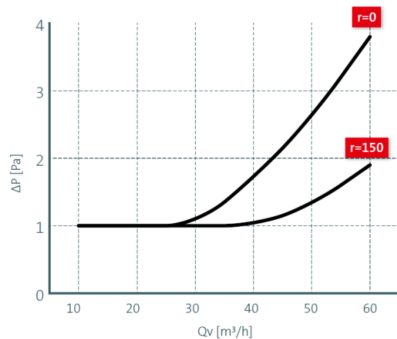
DN 90/75mm
