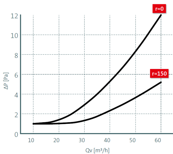
DN75/63mm
